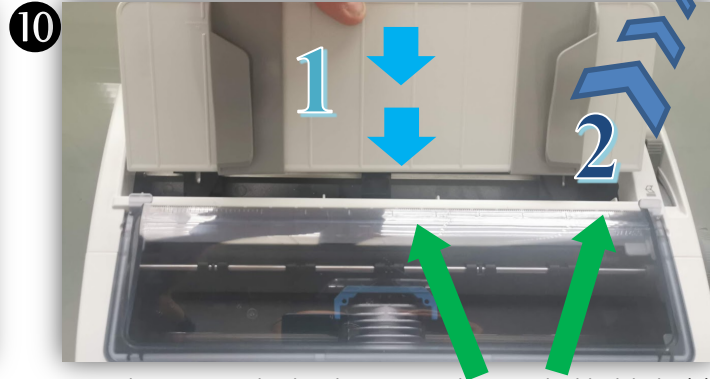
Insert the paper guide plate by pressing down to the black bolts (1) and push it backwards upon fixed on the white bolts (2)
